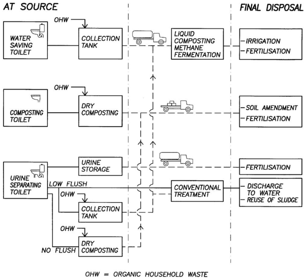
Figure 3: Logistics of blackwater and organic waste handling dependent of toilet type (Jenssen & Etnier 1997)
