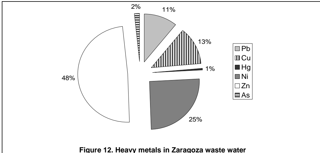
Figure 12. Heavy metals in Zaragoza waste water
